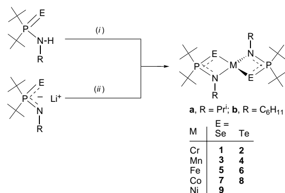
Scheme 1 (i) [M\{N(\text{SiMe}_3)_2\}_2] , light petroleum, room temperature (r.t.); (ii) \text{CrCl}_2 , \text{FeCl}_2 or [\text{NiCl}_2(\text{PMe}_3)_2] , thf, r.t.
